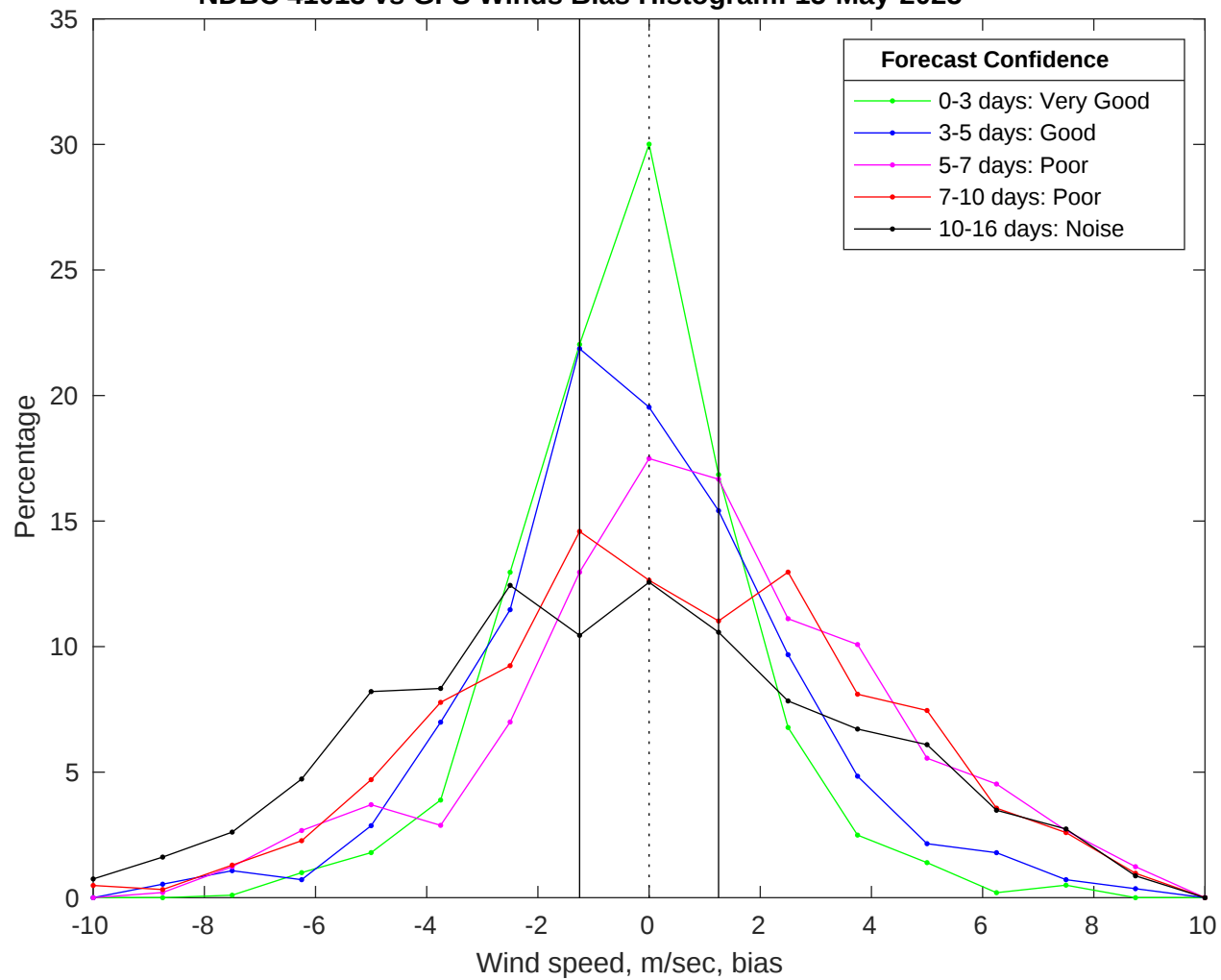
NDBC 41013 vs GFS Winds Bias Histogram: 15-May-2025
