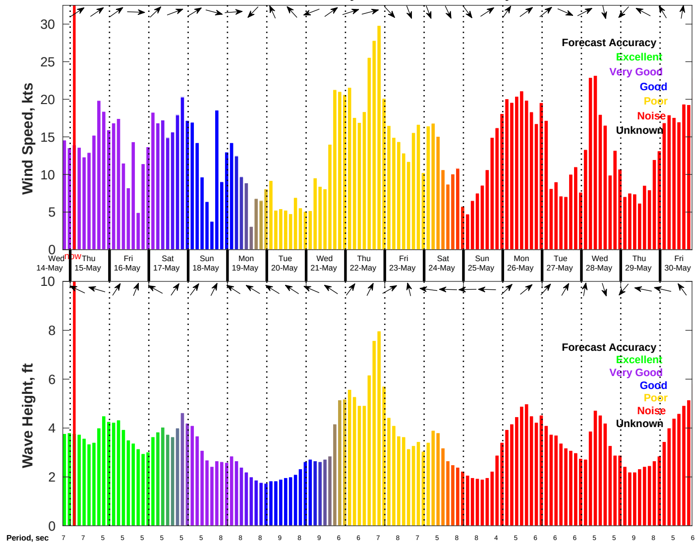
Wind & Wave Forecast for NDBC 41013 from 14-May-2025 19:00:00 to 30-May-2025 19:00:00
