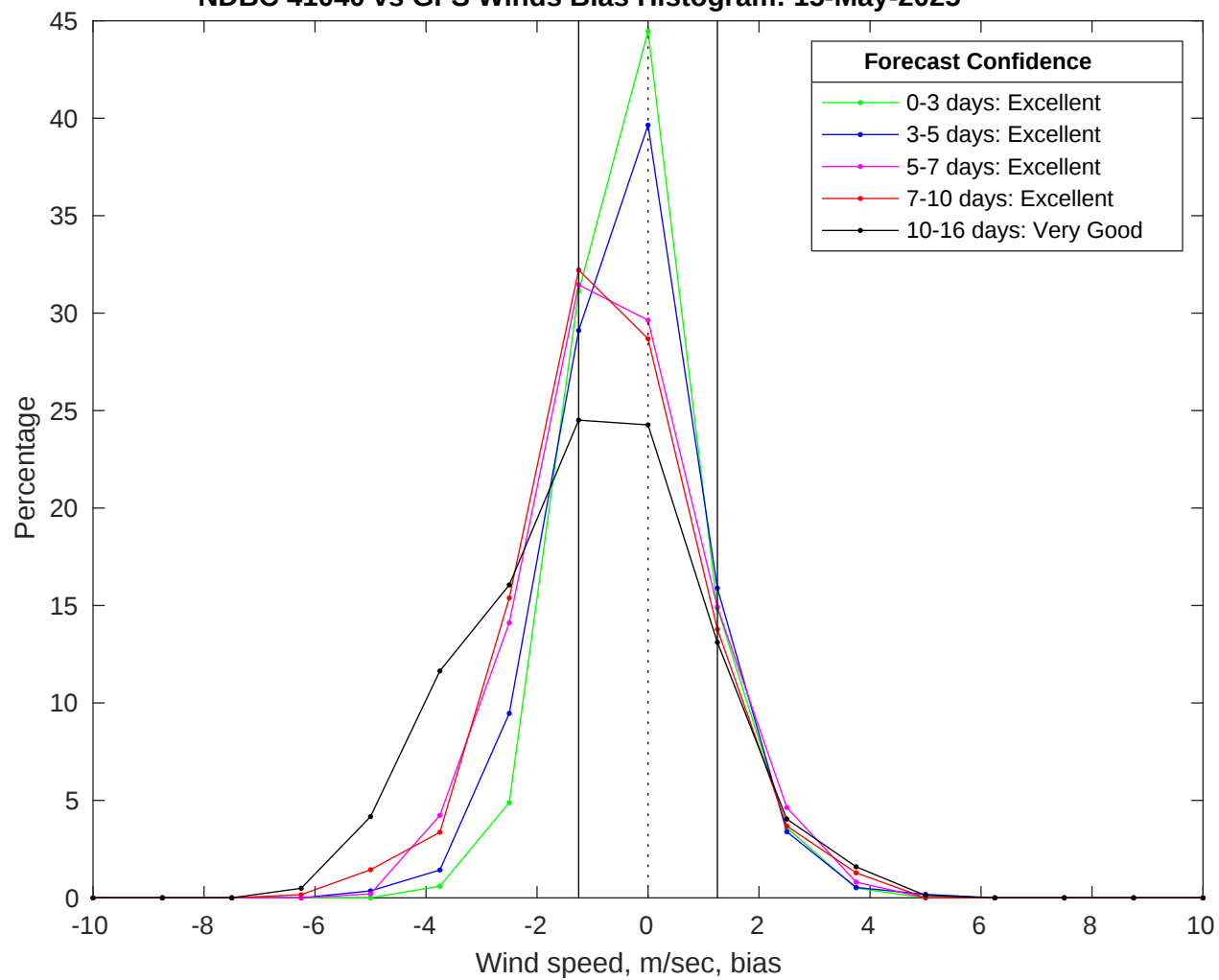
NDBC 41040 vs GFS Winds Bias Histogram: 15-May-2025
