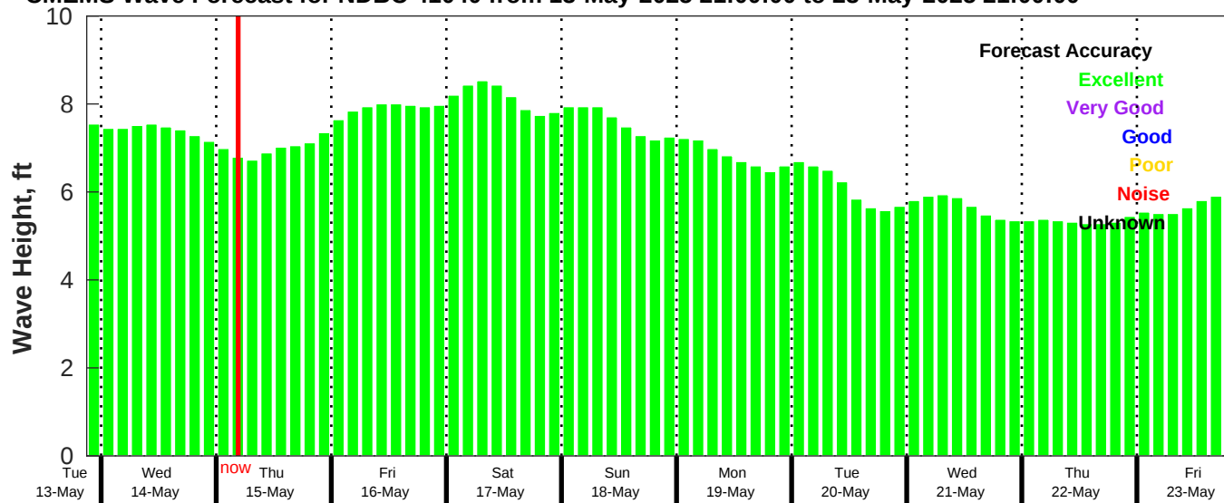
CMEMS Wave Forecast for NDBC 41040 from 13-May-2025 21:00:00 to 23-May-2025 21:00:00
