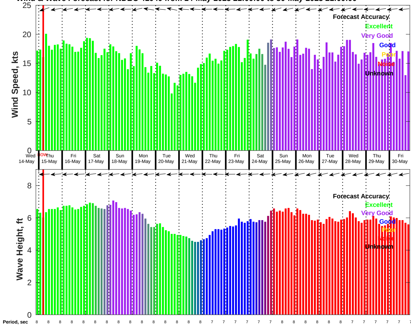
Wind & Wave Forecast for NDBC 41040 from 14-May-2025 21:00:00 to 30-May-2025 21:00:00
