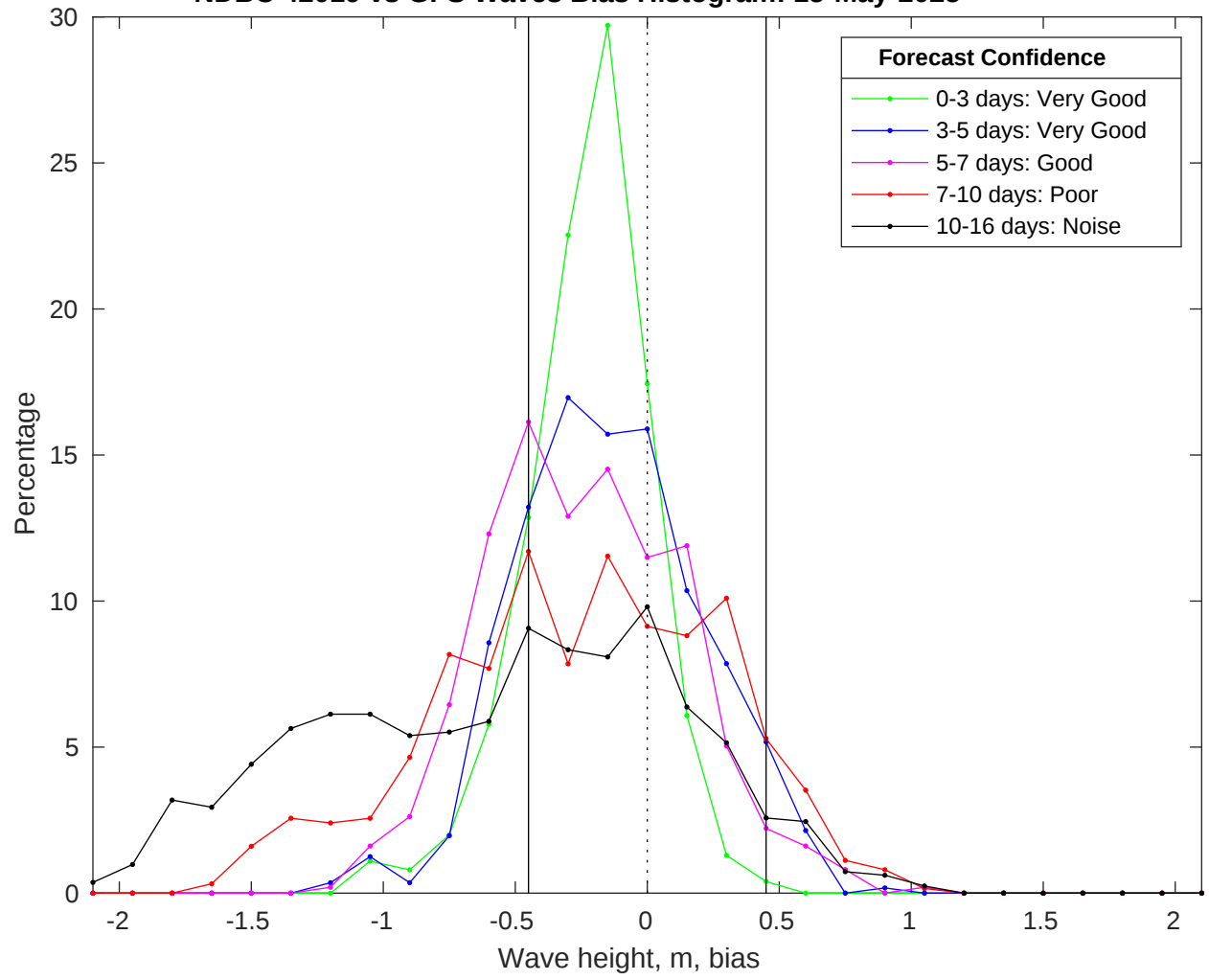
NDBC 42019 vs GFS Waves Bias Histogram: 15-May-2025
