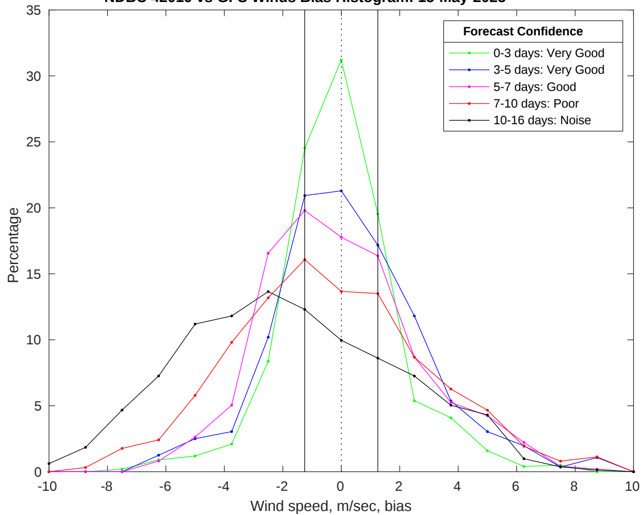
NDBC 42019 vs GFS Winds Bias Histogram: 15-May-2025
