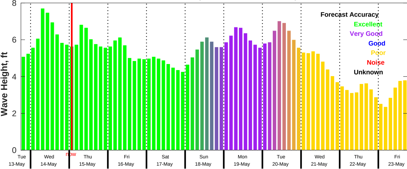
CMEMS Wave Forecast for NDBC 42019 from 13-May-2025 18:00:00 to 23-May-2025 18:00:00
