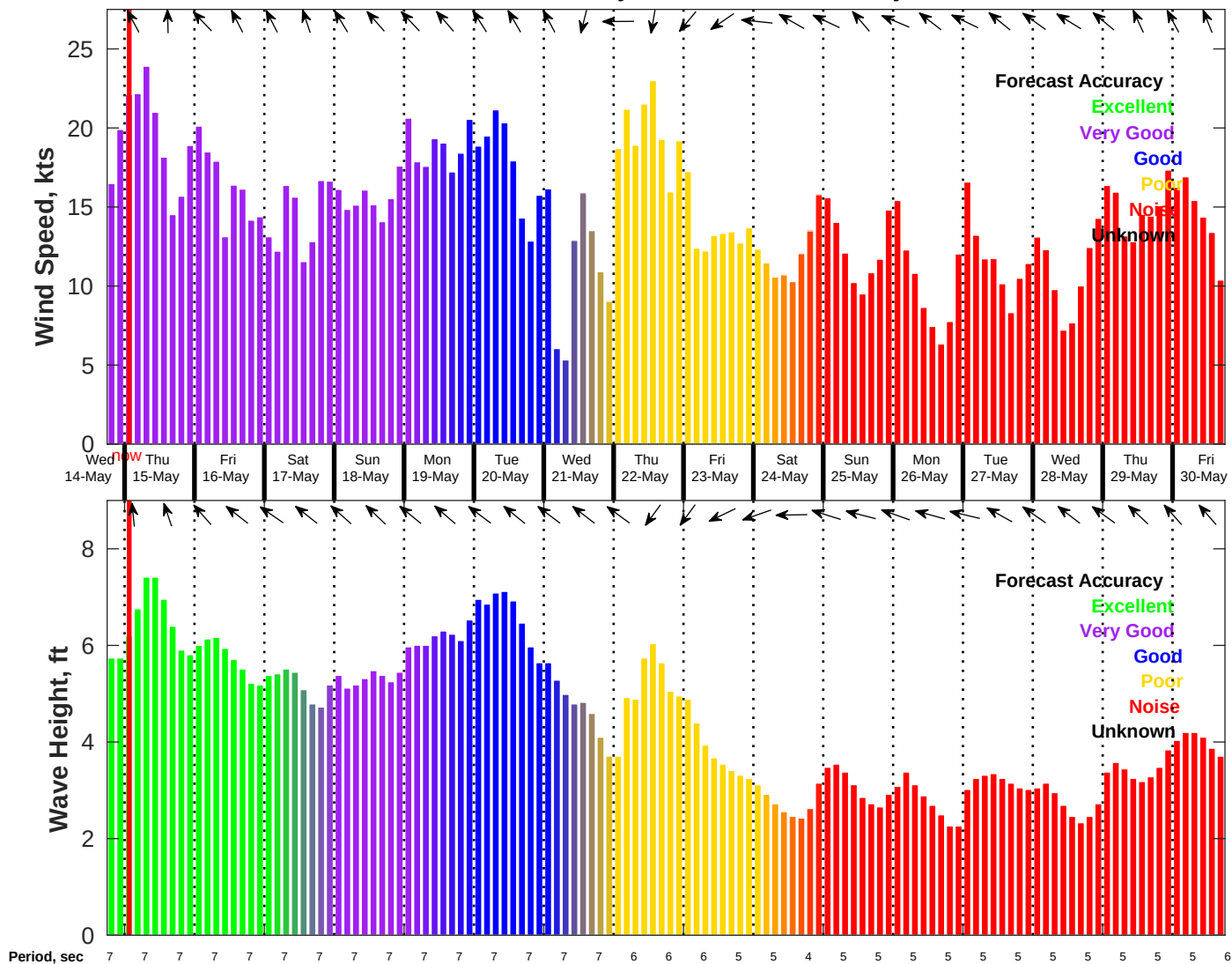
Wind & Wave Forecast for NDBC 42019 from 14-May-2025 18:00:00 to 30-May-2025 18:00:00
