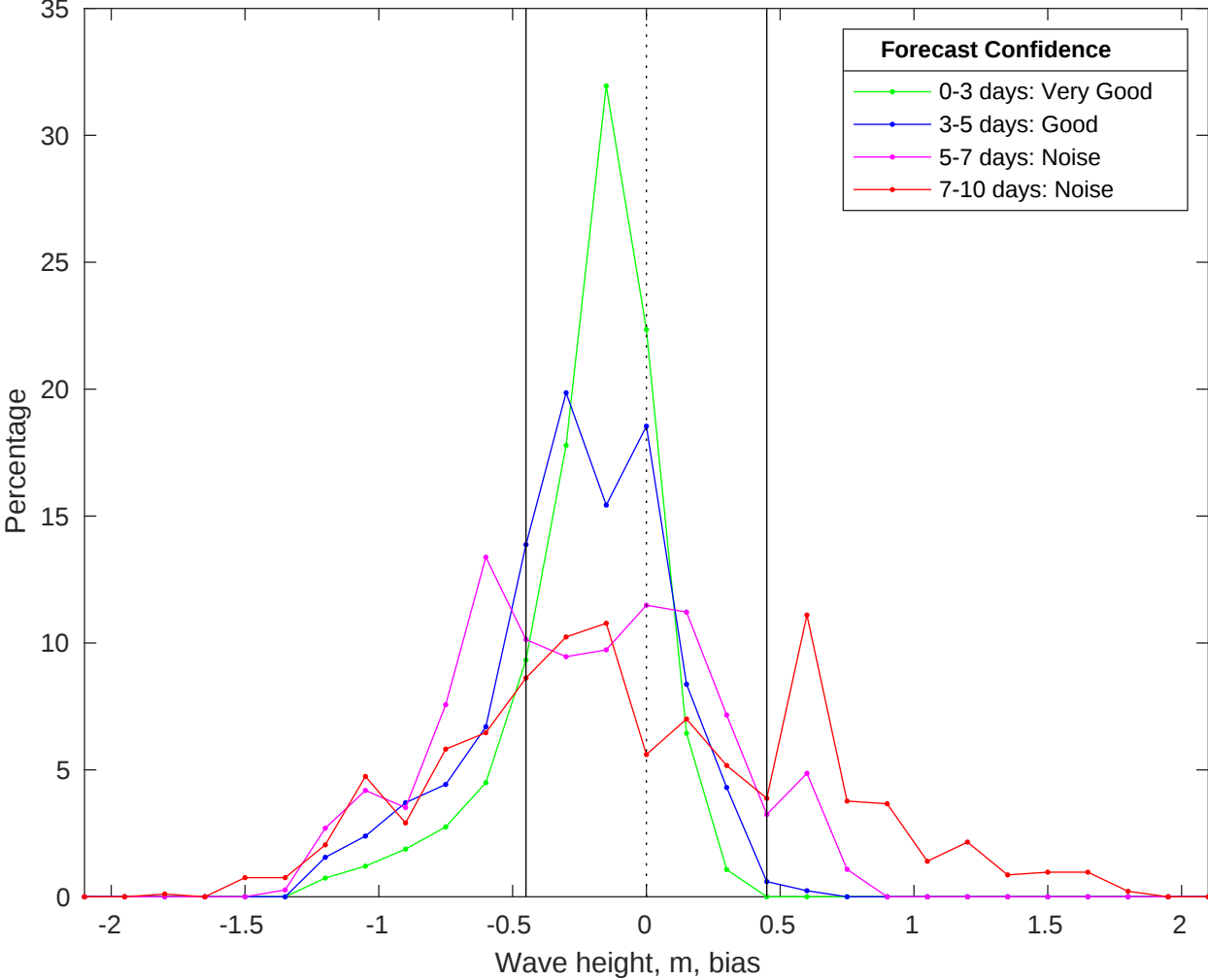
NDBC 42020 vs CMEMS Waves Bias Histogram: 15-May-2025
