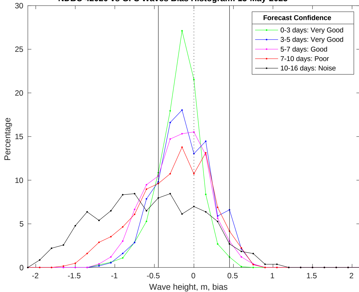
NDBC 42020 vs GFS Waves Bias Histogram: 15-May-2025
