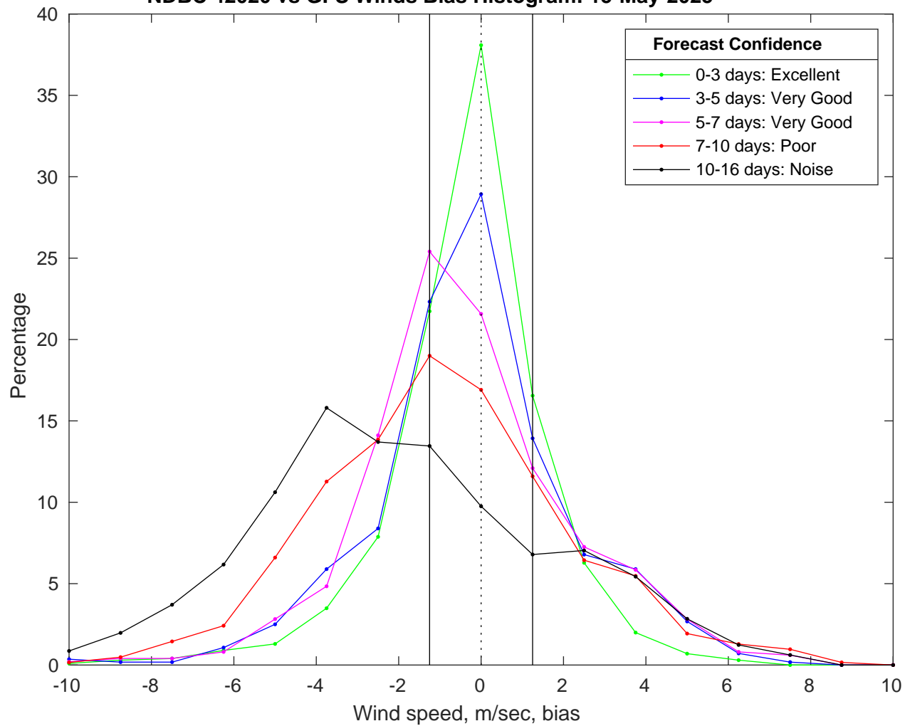
NDBC 42020 vs GFS Winds Bias Histogram: 15-May-2025
