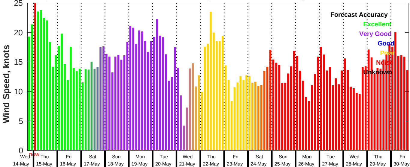
GFS Wind Speed Forecast for NDBC 42020 from 14-May-2025 18:00:00 to 30-May-2025 18:00:00
