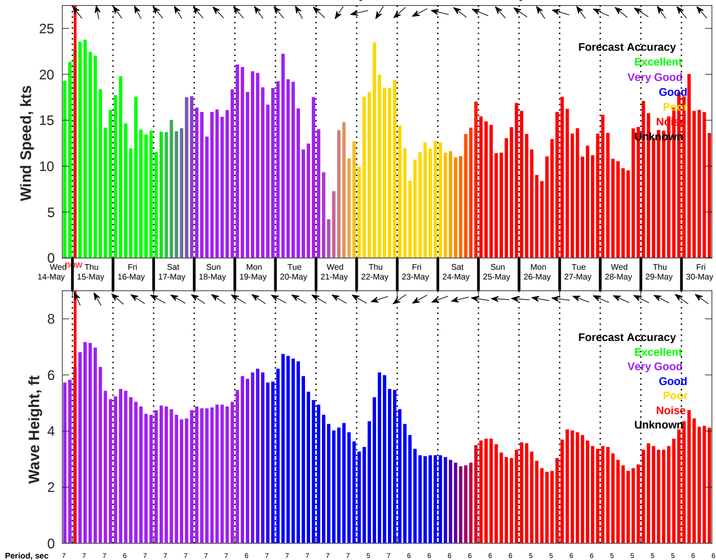
Wind & Wave Forecast for NDBC 42020 from 14-May-2025 18:00:00 to 30-May-2025 18:00:00
