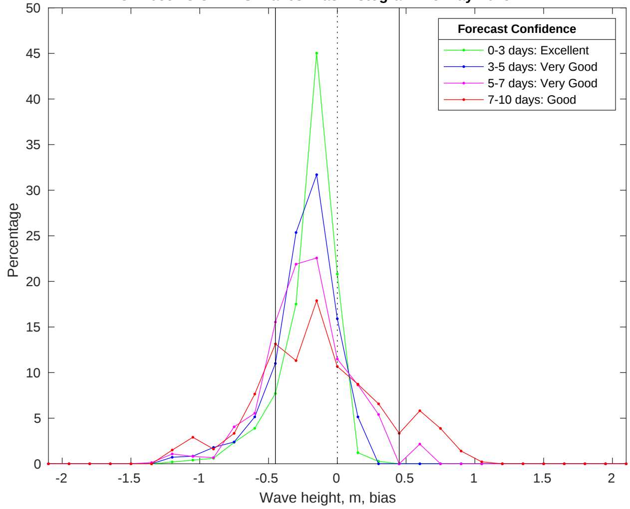
NDBC 42035 vs CMEMS Waves Bias Histogram: 15-May-2025
