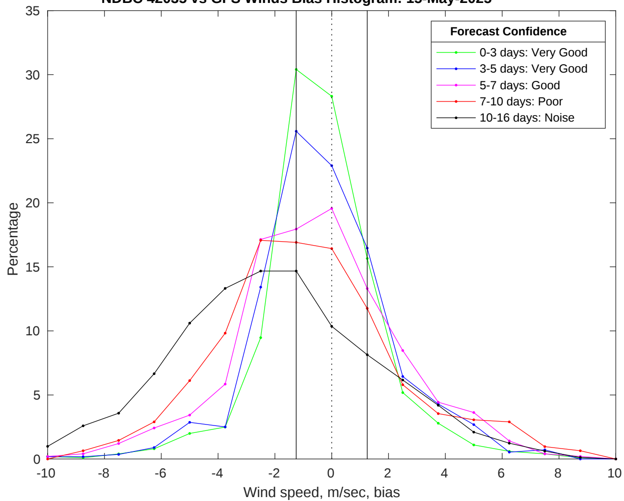
NDBC 42035 vs GFS Winds Bias Histogram: 15-May-2025
