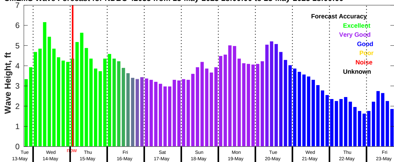
CMEMS Wave Forecast for NDBC 42035 from 13-May-2025 18:00:00 to 23-May-2025 18:00:00
