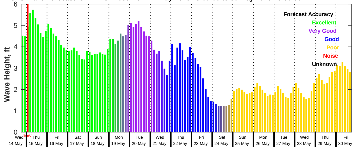
GFS Wave Forecast for NDBC 42035 from 14-May-2025 18:00:00 to 30-May-2025 18:00:00
