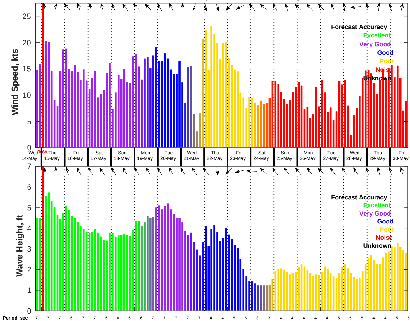
Wind & Wave Forecast for NDBC 42035 from 14-May-2025 18:00:00 to 30-May-2025 18:00:00
