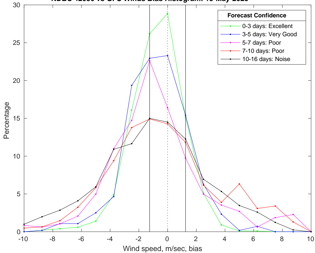
NDBC 42036 vs GFS Winds Bias Histogram: 15-May-2025
