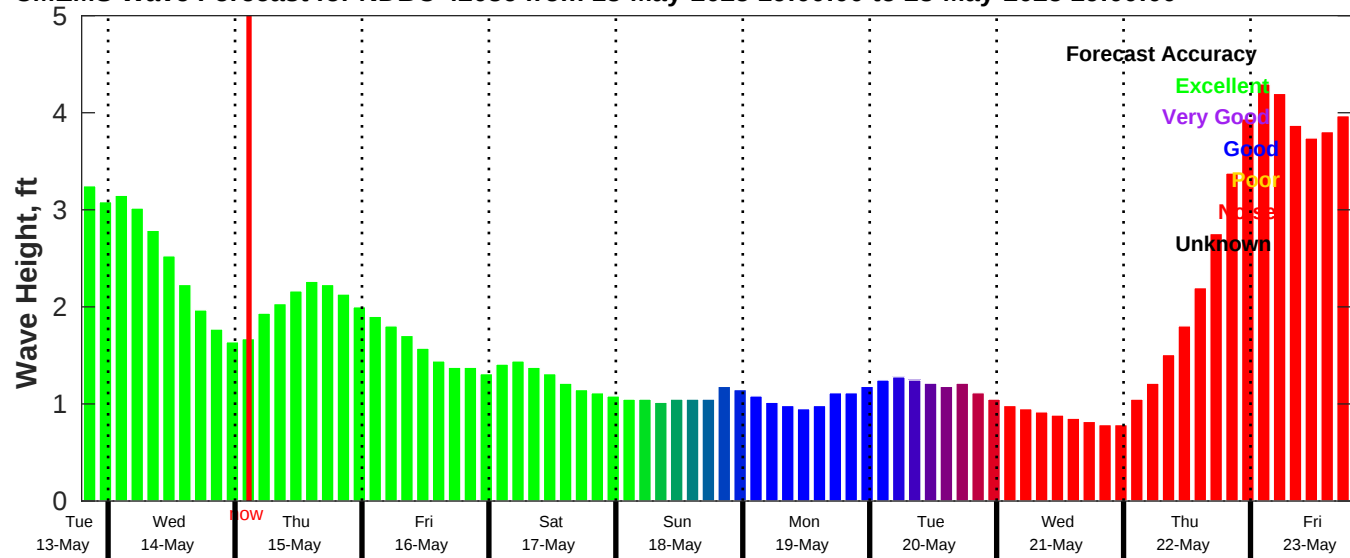
CMEMS Wave Forecast for NDBC 42036 from 13-May-2025 19:00:00 to 23-May-2025 19:00:00
