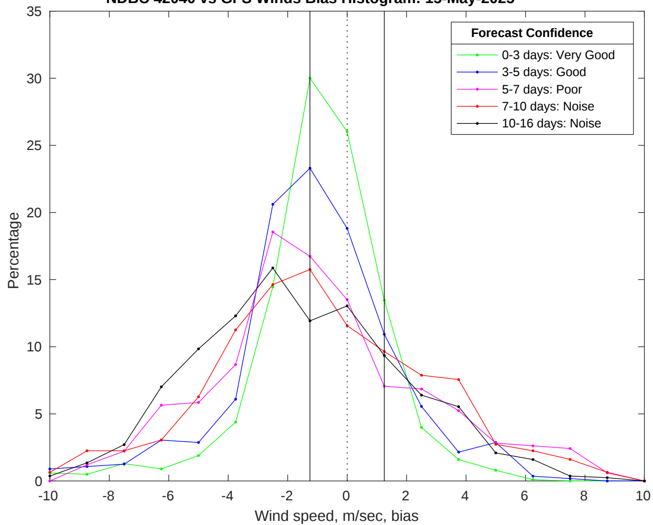
NDBC 42040 vs GFS Winds Bias Histogram: 15-May-2025
