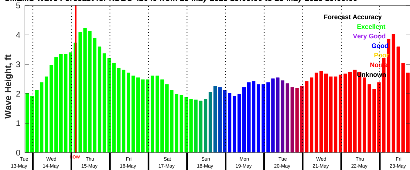
CMEMS Wave Forecast for NDBC 42040 from 13-May-2025 19:00:00 to 23-May-2025 19:00:00
