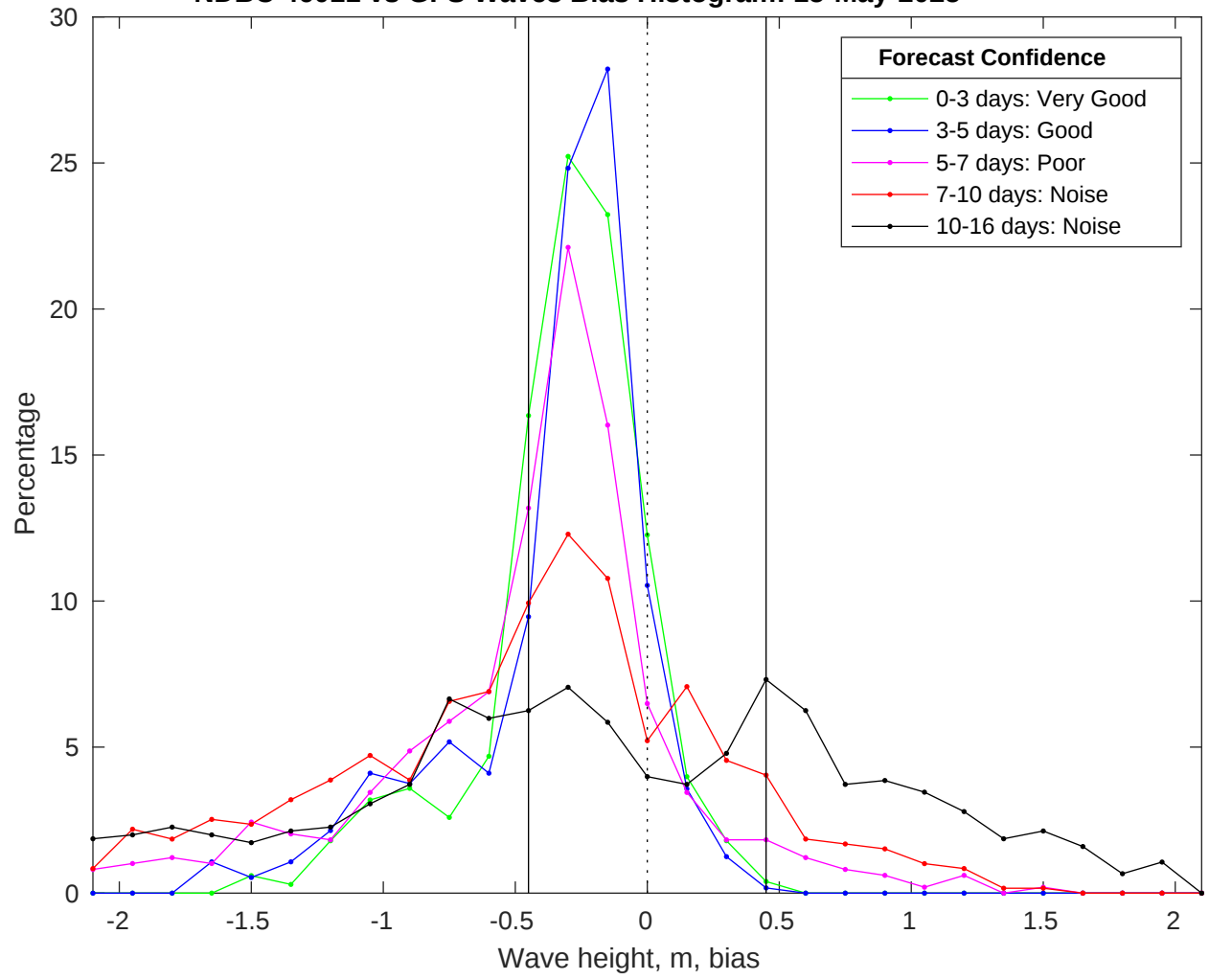
NDBC 46011 vs GFS Waves Bias Histogram: 15-May-2025
