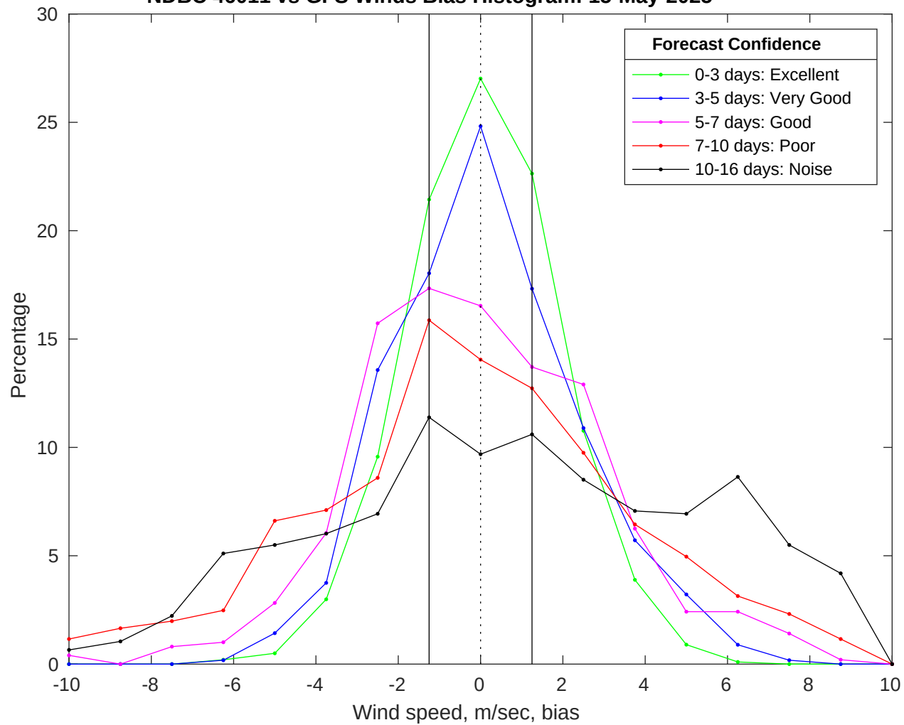
NDBC 46011 vs GFS Winds Bias Histogram: 15-May-2025
