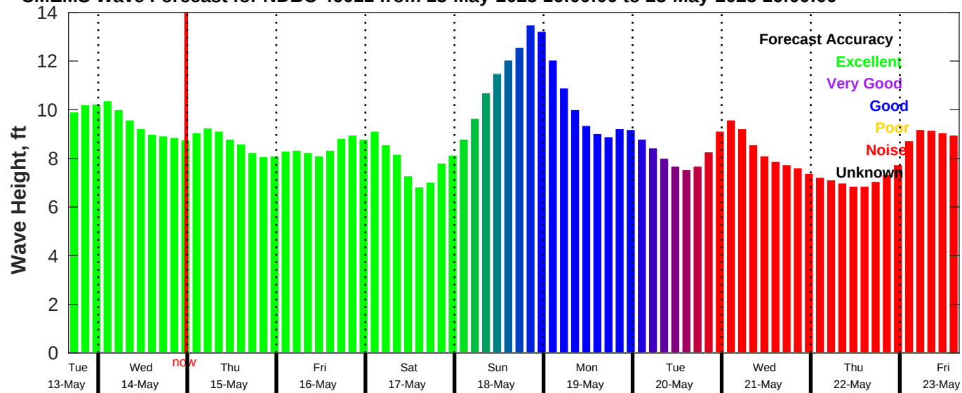
CMEMS Wave Forecast for NDBC 46011 from 13-May-2025 16:00:00 to 23-May-2025 16:00:00
