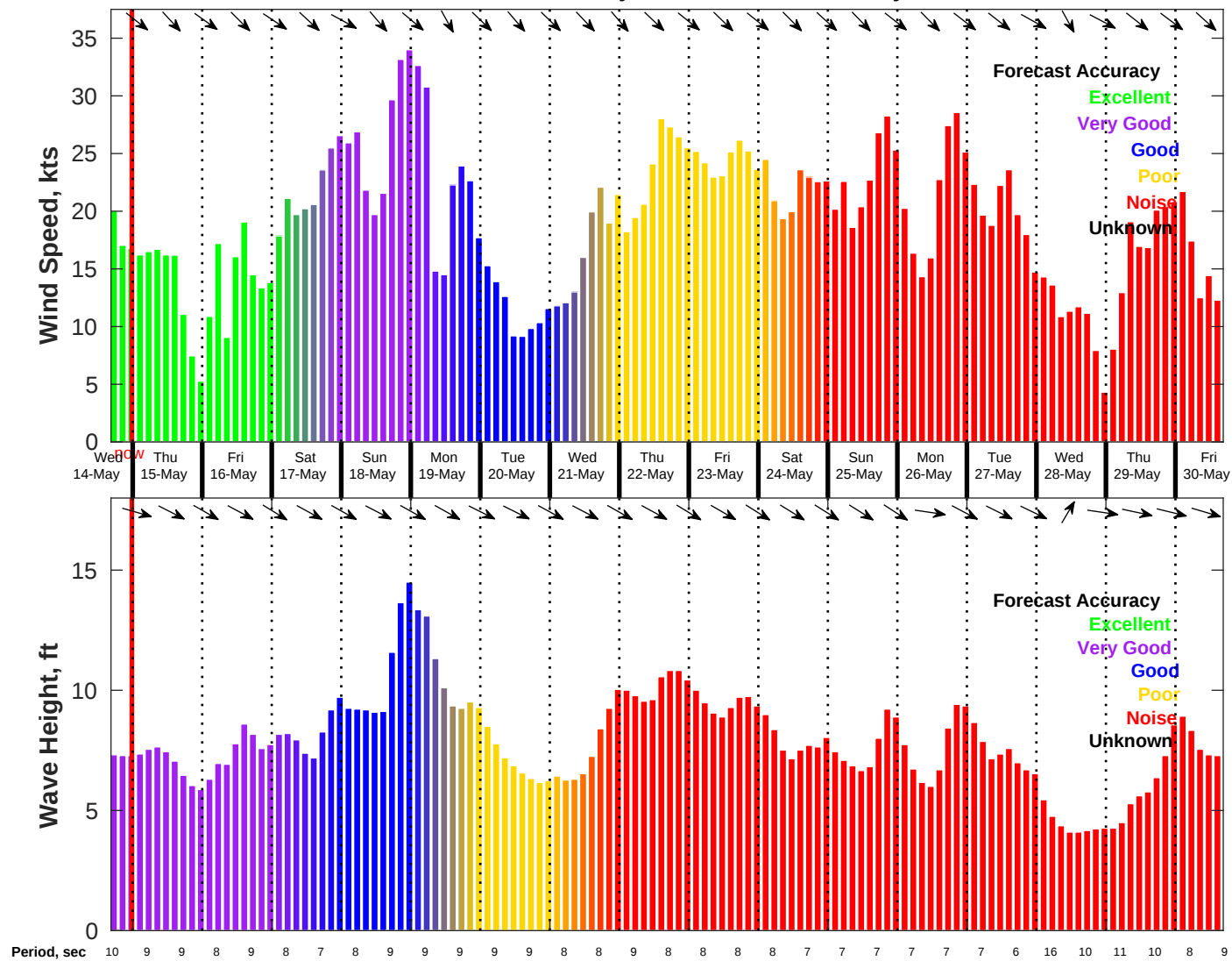
Wind & Wave Forecast for NDBC 46011 from 14-May-2025 16:00:00 to 30-May-2025 16:00:00
