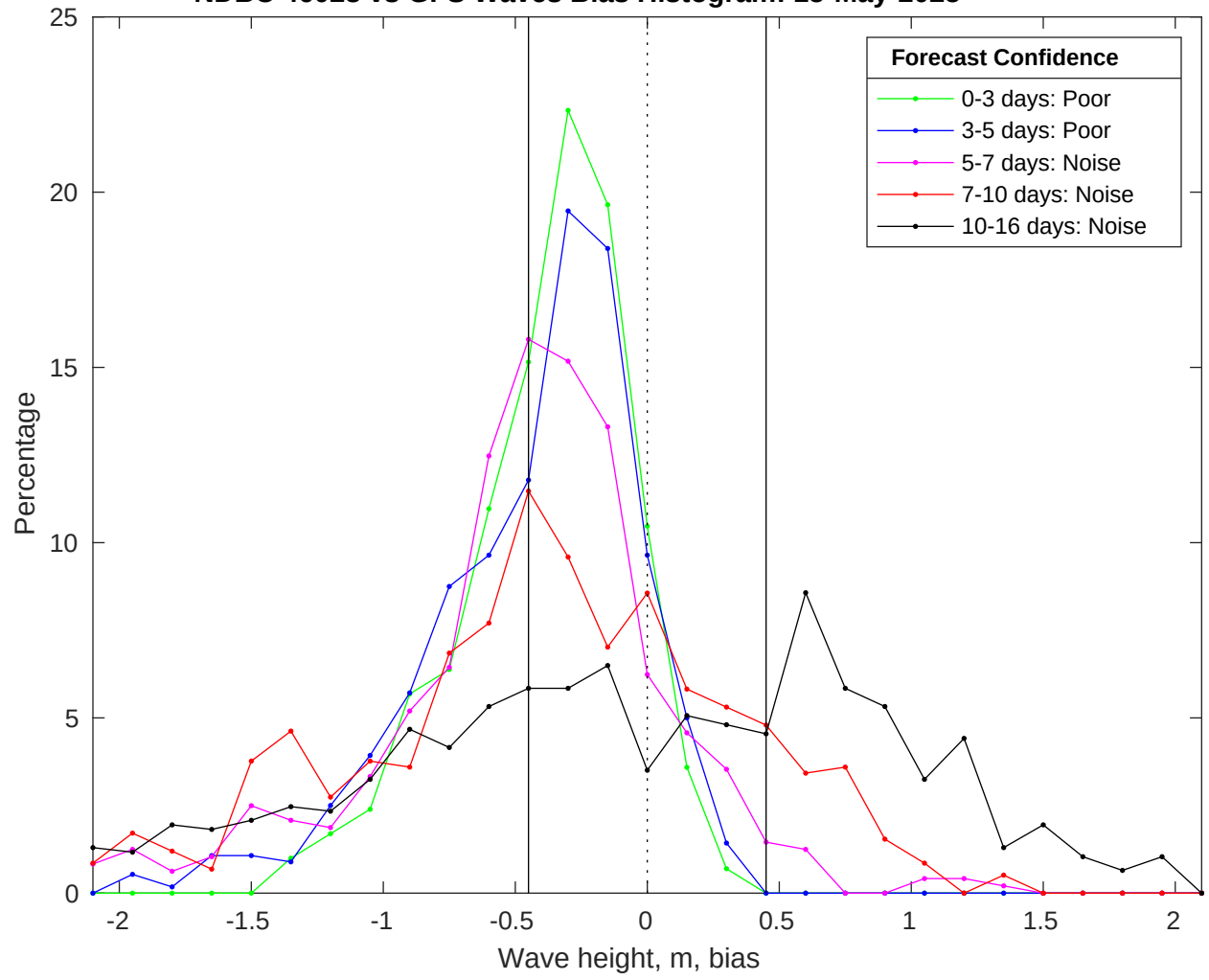
NDBC 46028 vs GFS Waves Bias Histogram: 15-May-2025
