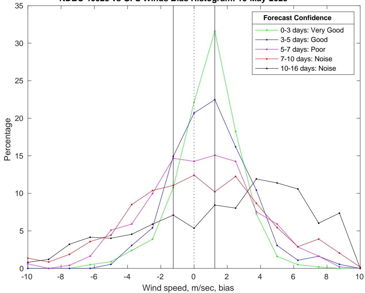
NDBC 46028 vs GFS Winds Bias Histogram: 15-May-2025
