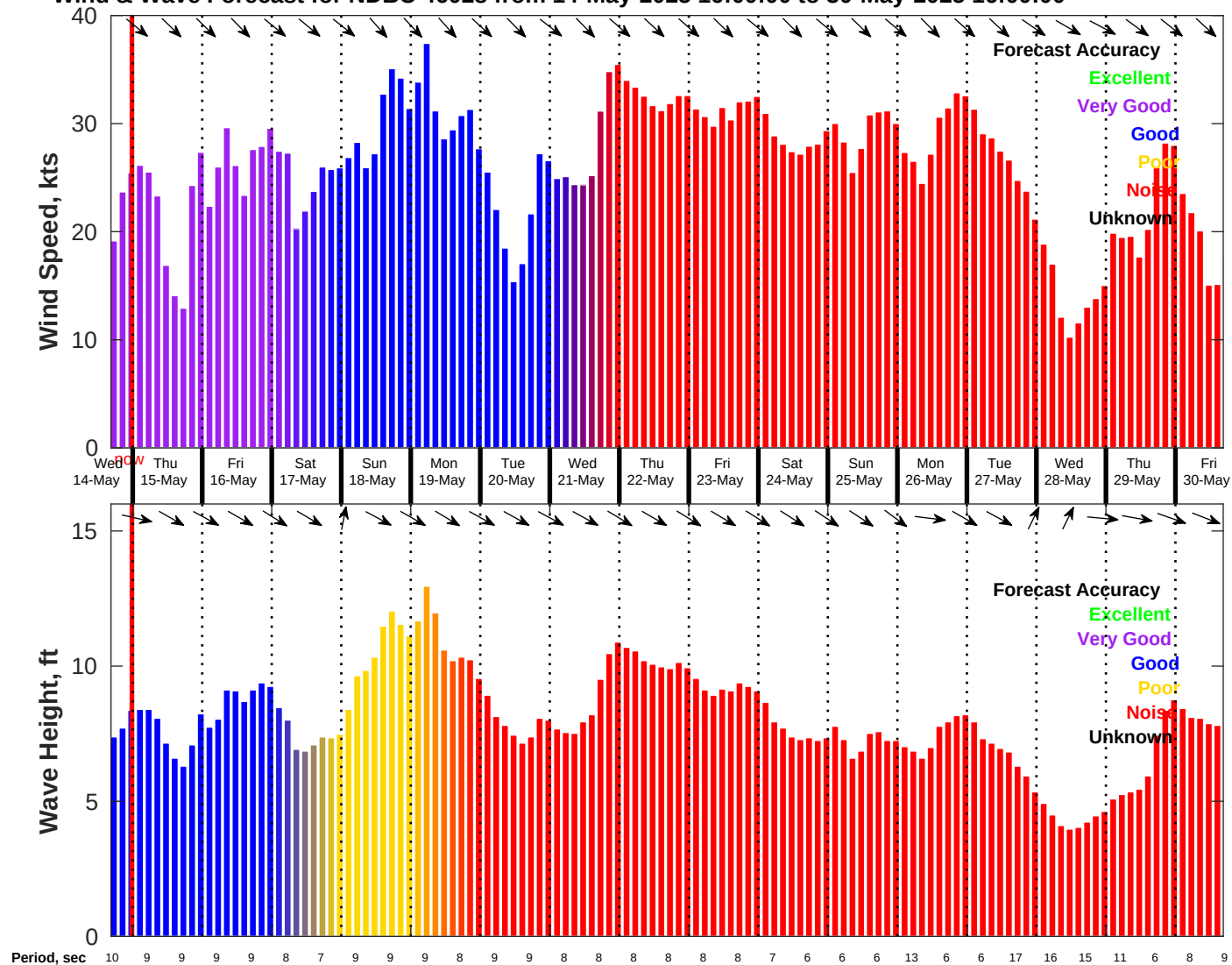
Wind & Wave Forecast for NDBC 46028 from 14-May-2025 16:00:00 to 30-May-2025 16:00:00
