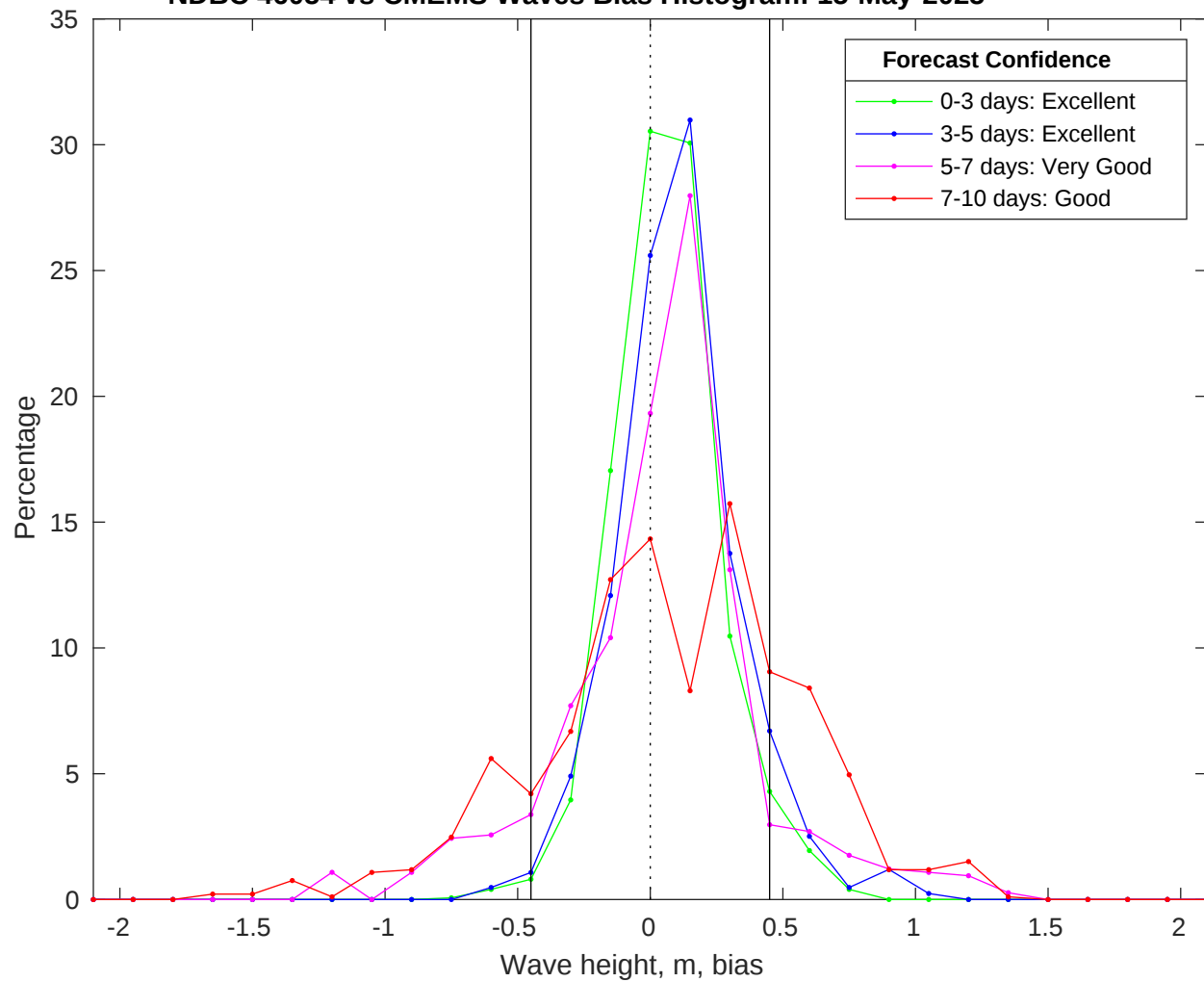
NDBC 46054 vs CMEMS Waves Bias Histogram: 15-May-2025
