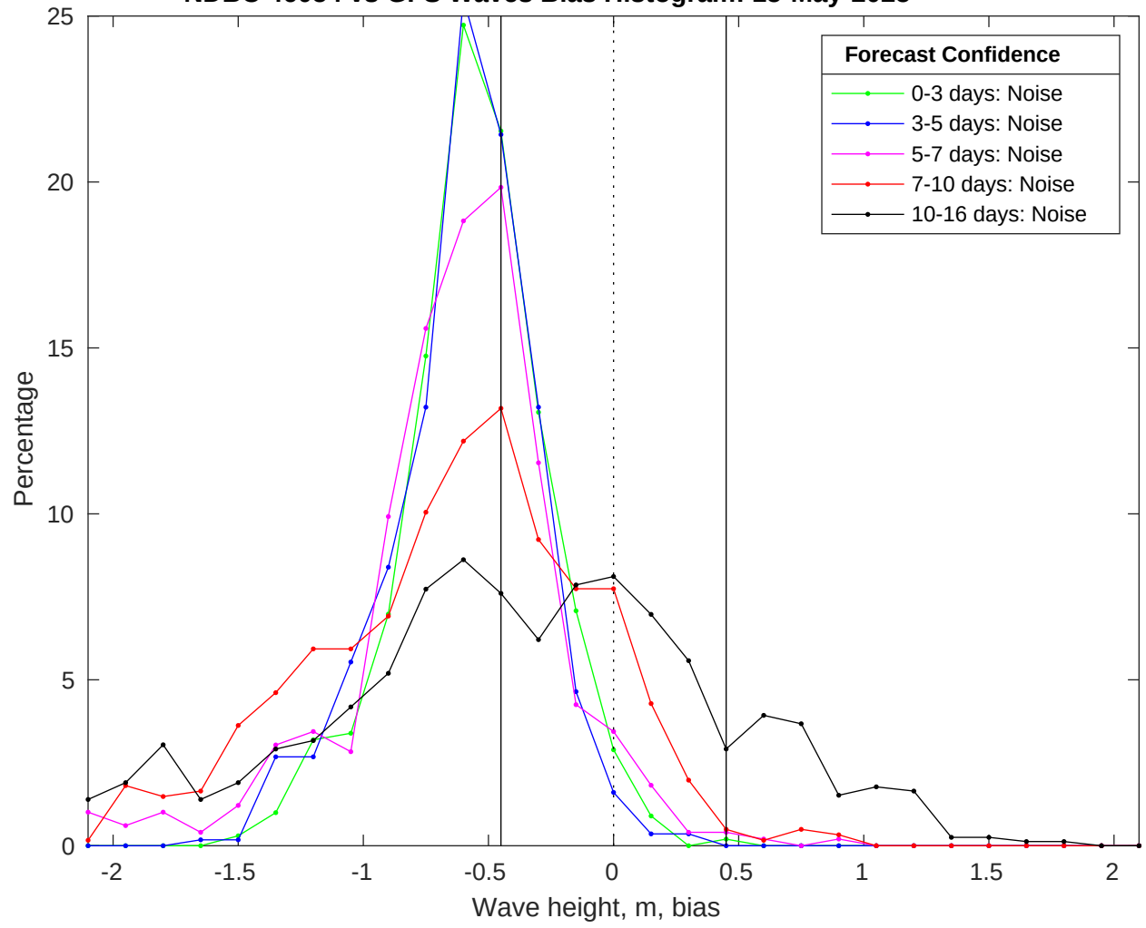
NDBC 46054 vs GFS Waves Bias Histogram: 15-May-2025
