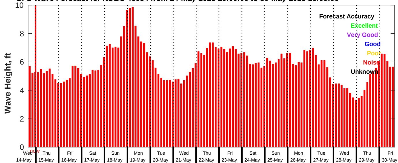
GFS Wave Forecast for NDBC 46054 from 14-May-2025 16:00:00 to 30-May-2025 16:00:00
