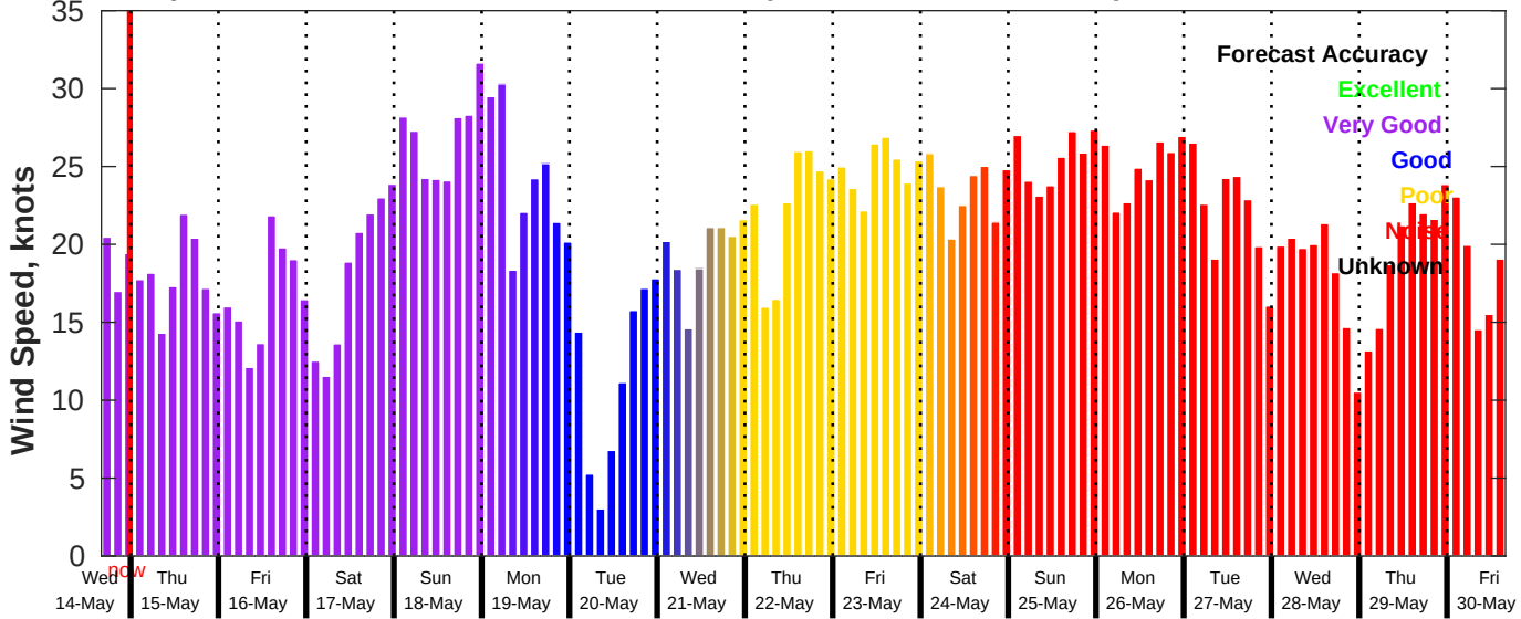
GFS Wind Speed Forecast for NDBC 46054 from 14-May-2025 16:00:00 to 30-May-2025 16:00:00
