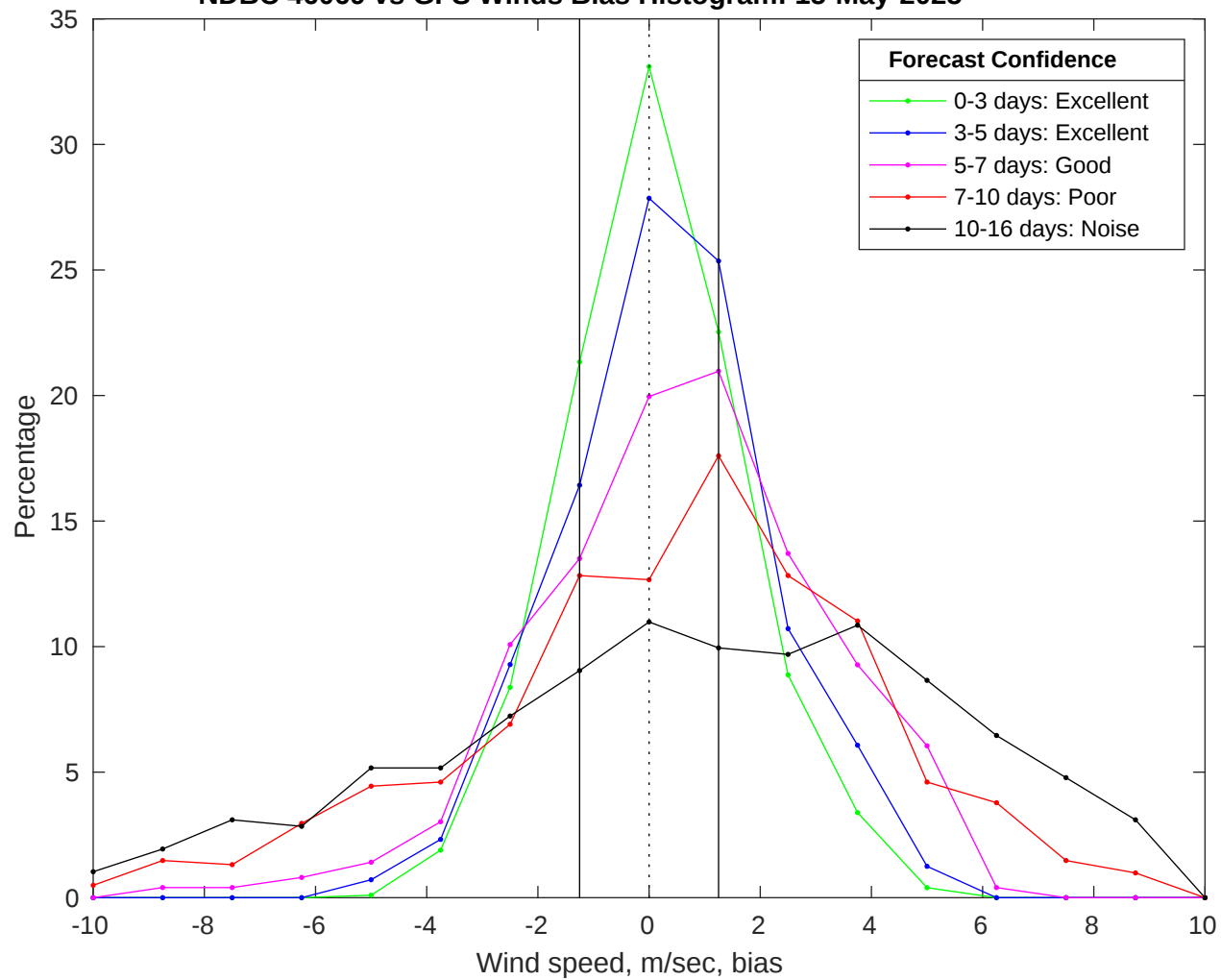
NDBC 46069 vs GFS Winds Bias Histogram: 15-May-2025
