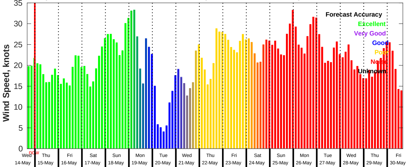
GFS Wind Speed Forecast for NDBC 46069 from 14-May-2025 16:00:00 to 30-May-2025 16:00:00
