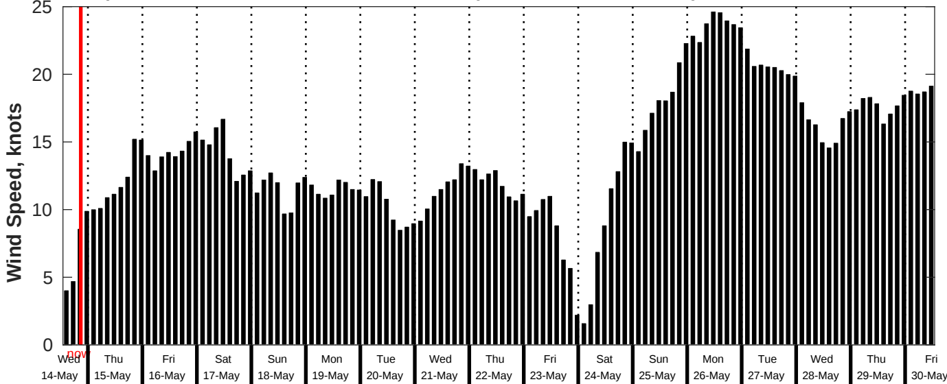
GFS Wind Speed Forecast for NDBC 51209 from 14-May-2025 13:00:00 to 30-May-2025 13:00:00
