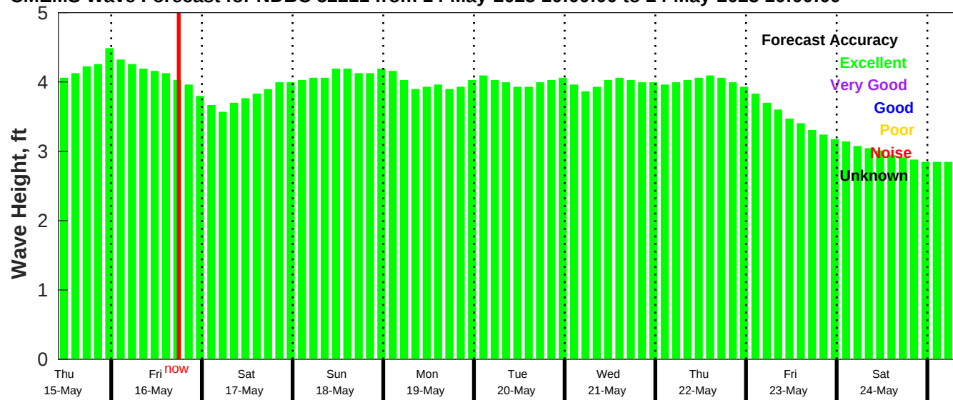
CMEMS Wave Forecast for NDBC 52211 from 14-May-2025 10:00:00 to 24-May-2025 10:00:00
