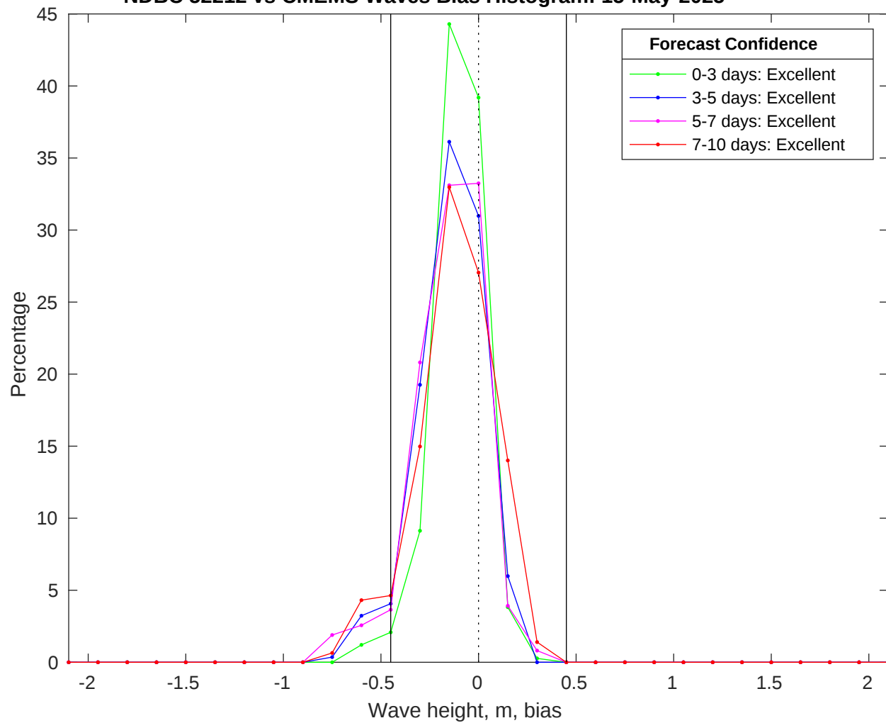
NDBC 52212 vs CMEMS Waves Bias Histogram: 15-May-2025
