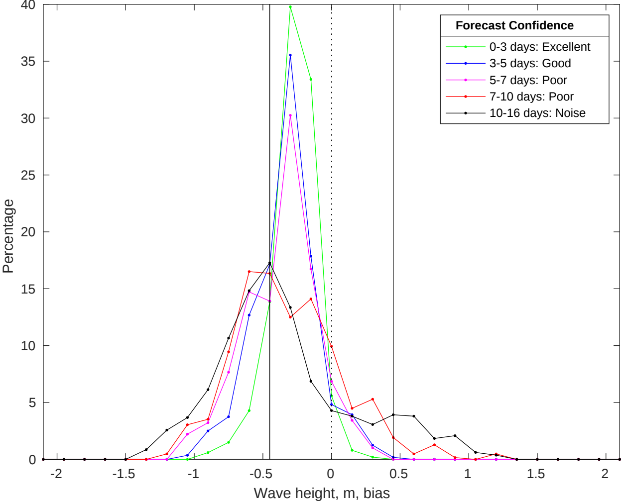
NDBC 52212 vs GFS Waves Bias Histogram: 15-May-2025
