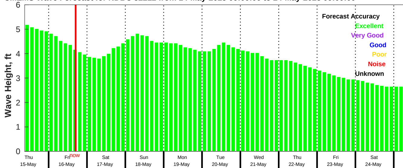
CMEMS Wave Forecast for NDBC 52212 from 14-May-2025 09:00:00 to 24-May-2025 09:00:00
