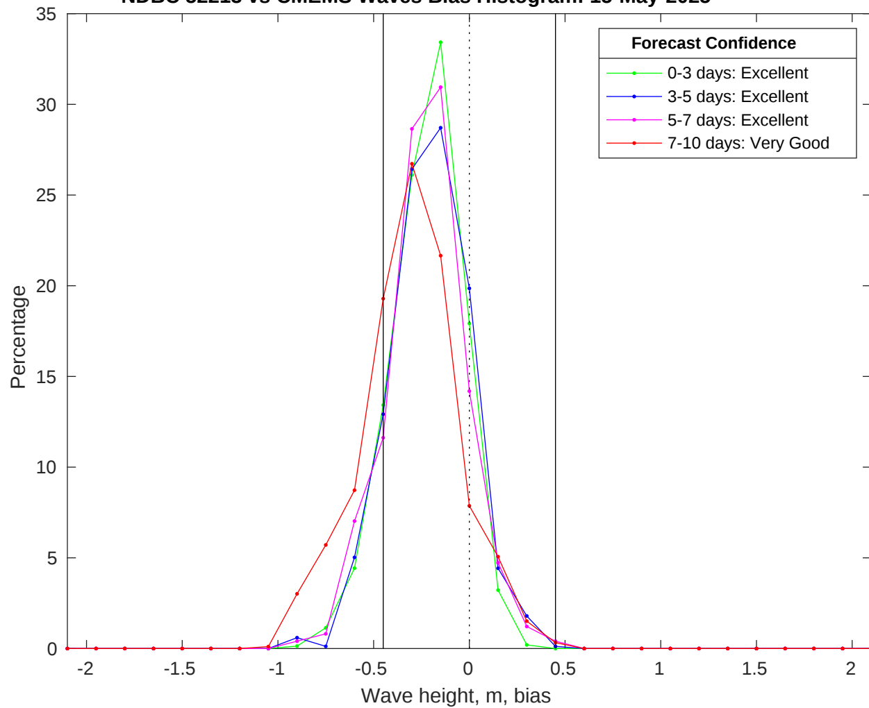
NDBC 52213 vs CMEMS Waves Bias Histogram: 15-May-2025
