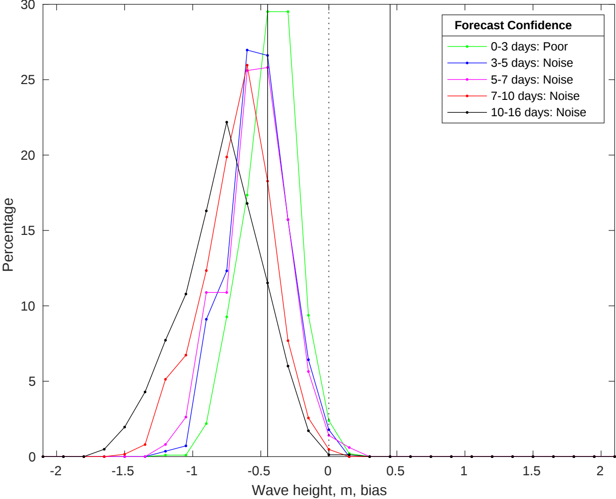
NDBC 52213 vs GFS Waves Bias Histogram: 15-May-2025
