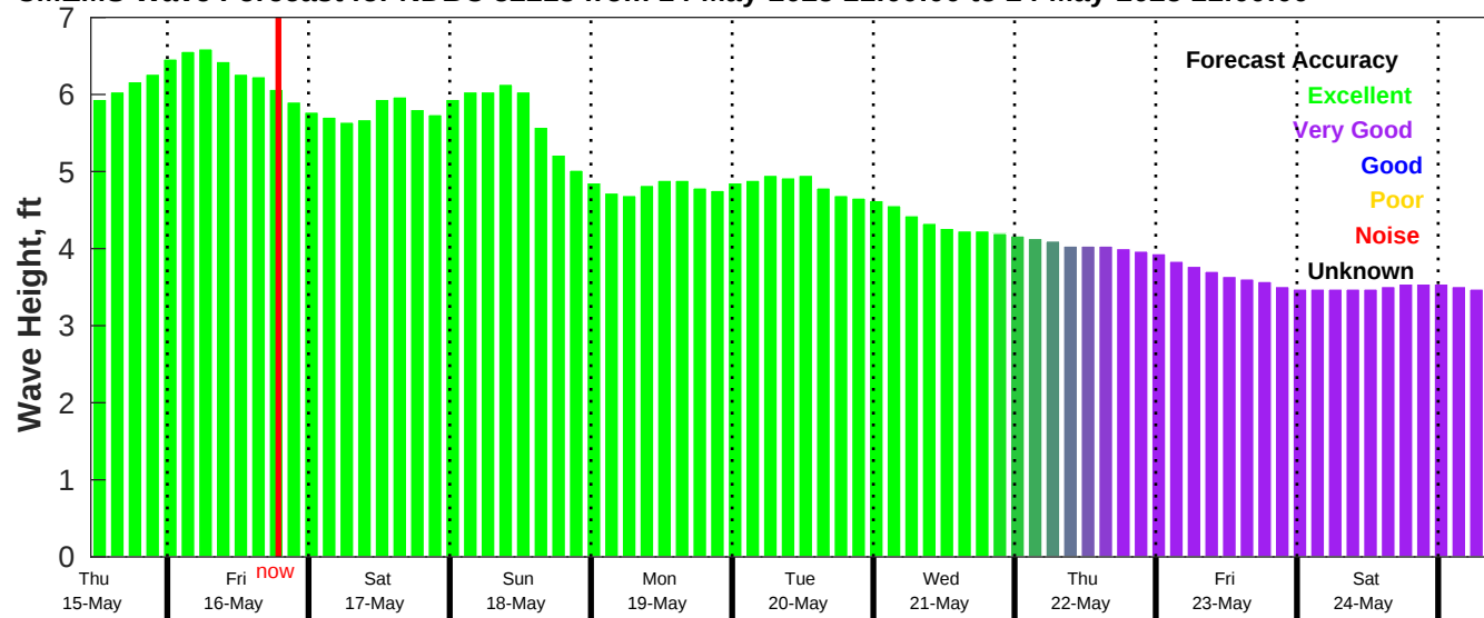
CEEMS Wave Forecast for NDBC 52213 from 14-May-2025 11:00:00 to 24-May-2025 11:00:00
