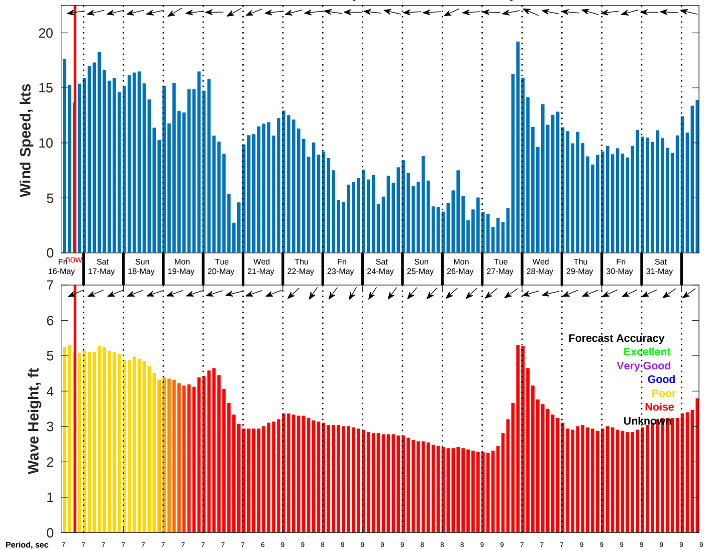
Wind & Wave Forecast for NDBC 52213 from 15-May-2025 11:00:00 to 31-May-2025 11:00:00
