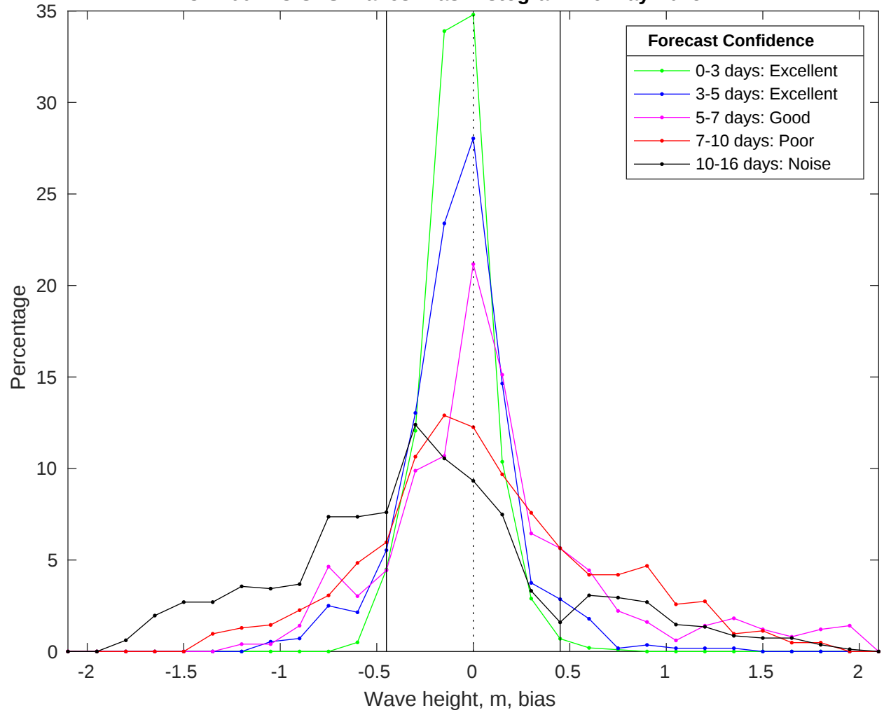
NDBC 41004 vs GFS Waves Bias Histogram: 16-May-2025
