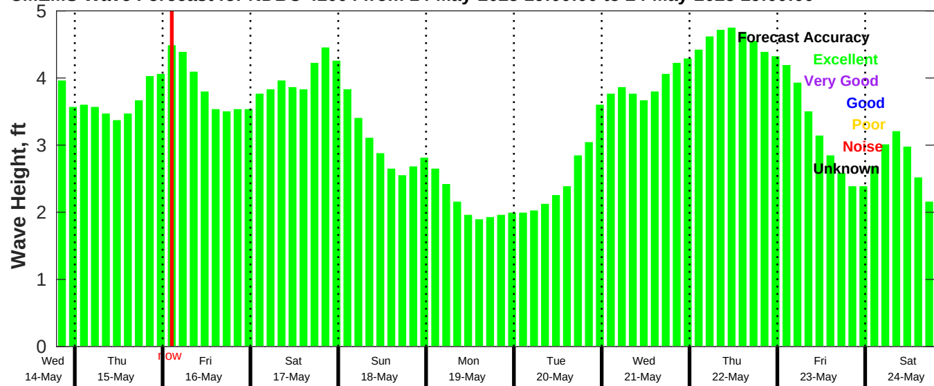
CMEMS Wave Forecast for NDBC 41004 from 14-May-2025 19:00:00 to 24-May-2025 19:00:00
