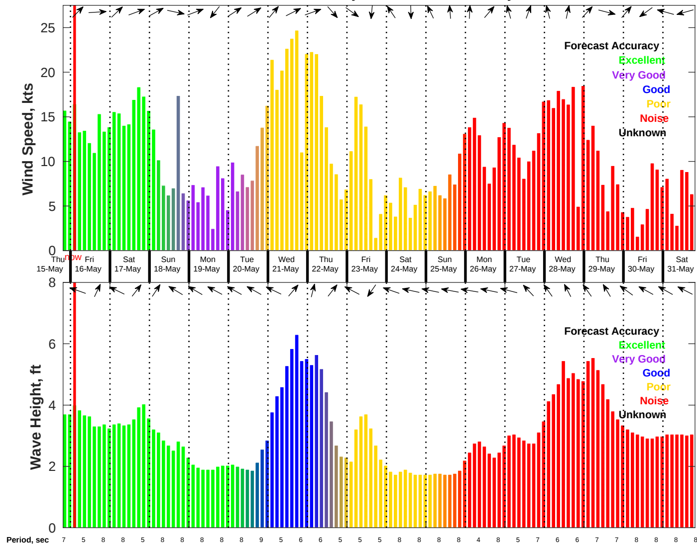
Wind & Wave Forecast for NDBC 41004 from 15-May-2025 19:00:00 to 31-May-2025 19:00:00
