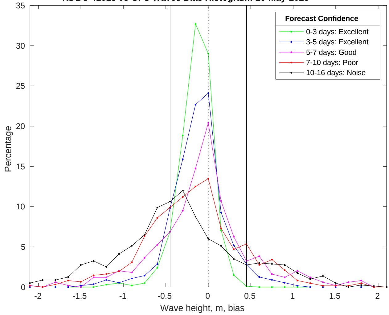
NDBC 41013 vs GFS Waves Bias Histogram: 16-May-2025
