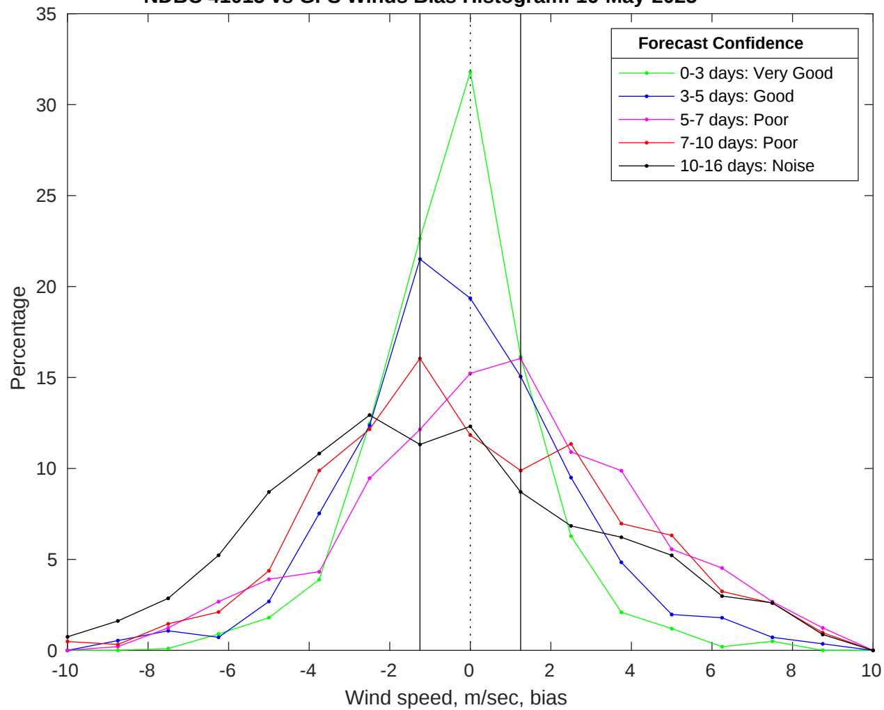
NDBC 41013 vs GFS Winds Bias Histogram: 16-May-2025
